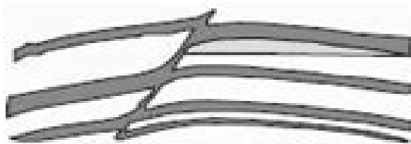
(a) Sealing To non-sealing faults
