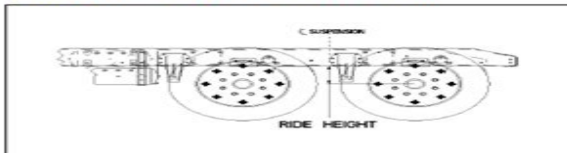
Ride Height Measurement (Location for Tandem Axles Shown)
