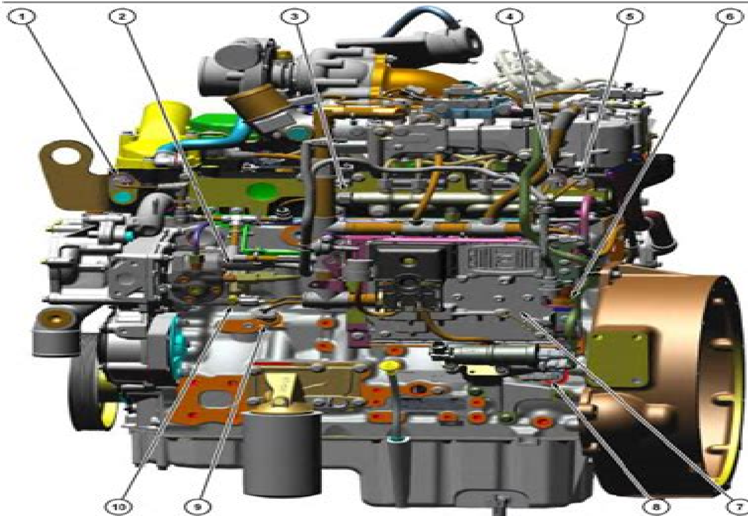
Illustration 4 Sensor locations on the left side of the engine
