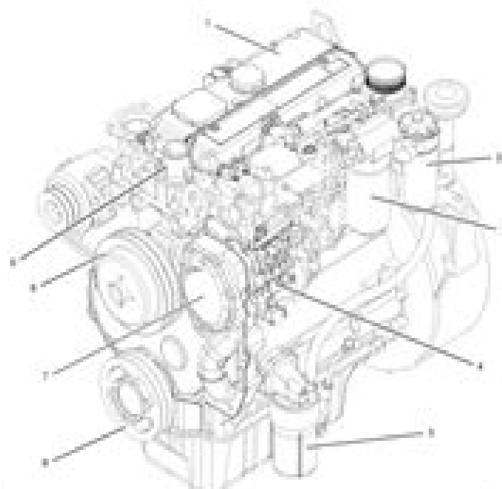
Illustration 1 (1) Valve mechanism cover (2) Governor housing (3) Fuel filter (4) Fuel injection pump (5) Engine oil filter (6) Governor body (7) Water pump (8) Fan pulley (9) Water temperature regulator housing
