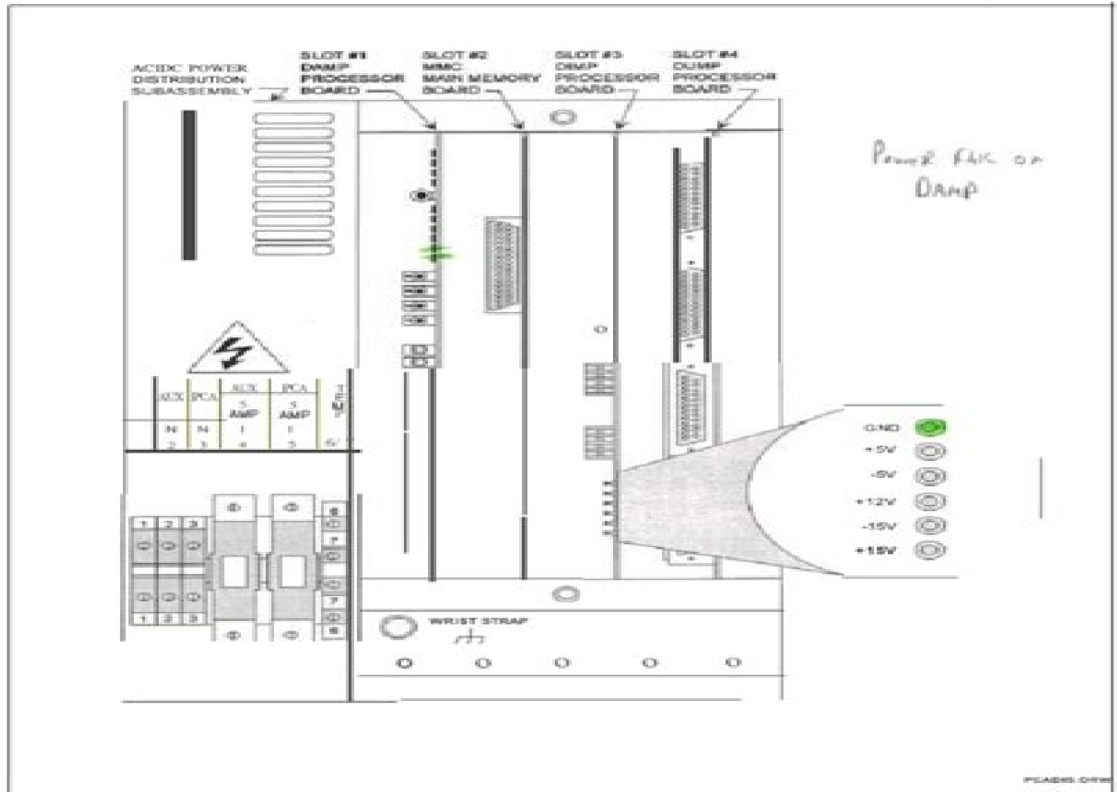
Figure 4.1.5 peA Voltage Reference Points
