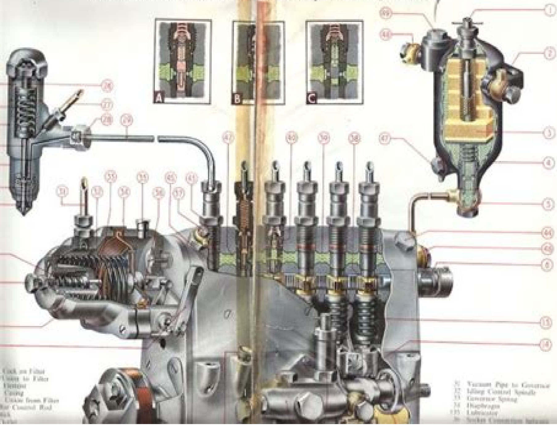
FIG. 20. GHOST DRAWING OF FUEL INJECTION EQUIPMENT
