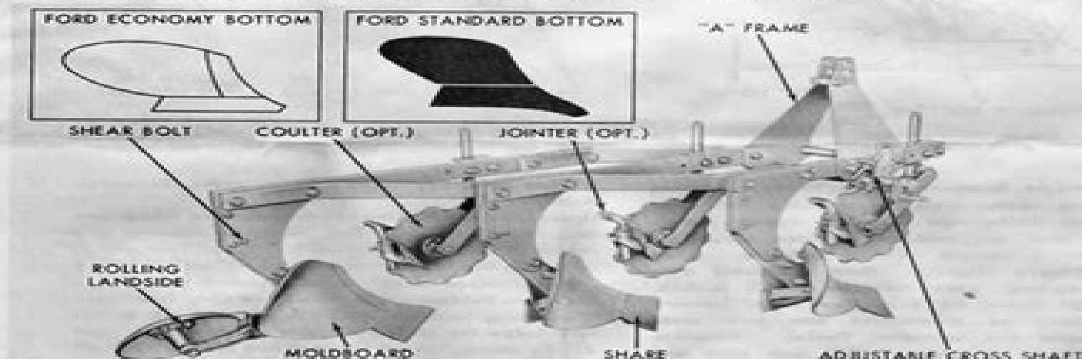
Figure 1 - Ford Three Bottom Moldboard Plow
