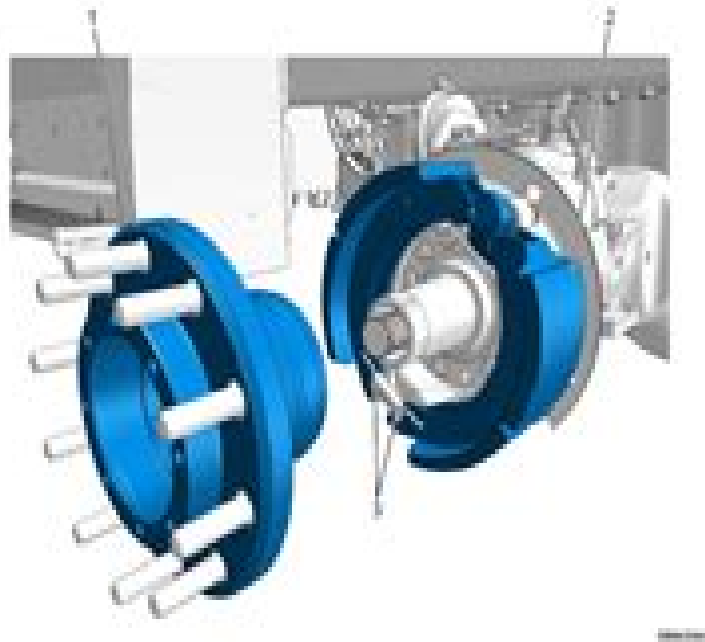
Figure 54 Wheel Hub and Brakes
