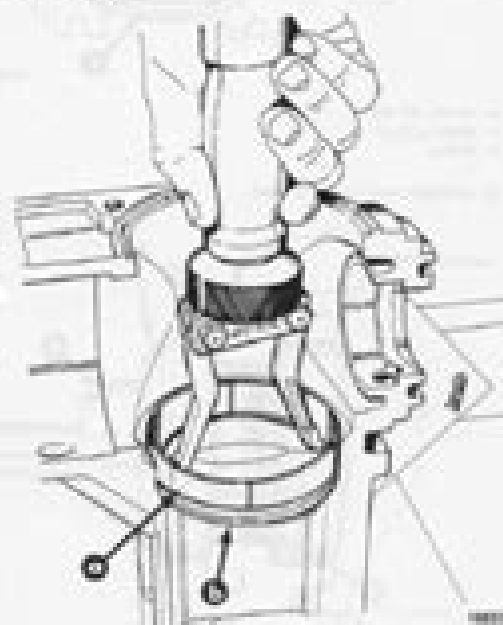
A - Bearing Cap B - Shim
