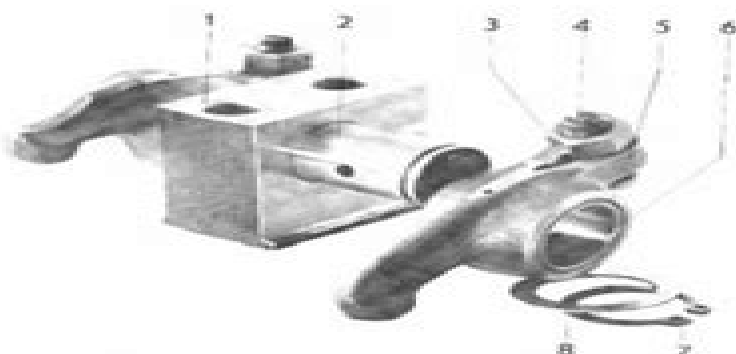
Fig. 13. Rocker arm mechanism
