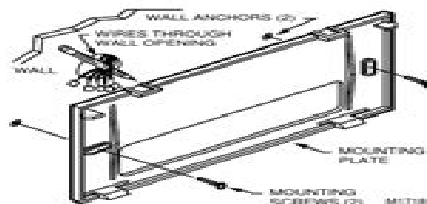
Fig. 2. Mounting plate installation.
